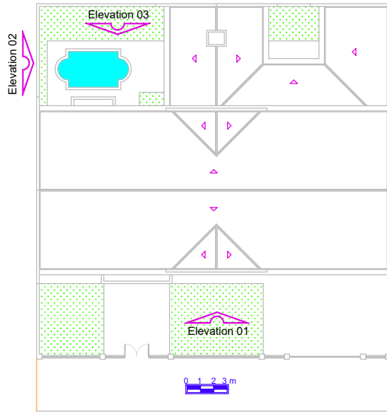
Roof Plan
