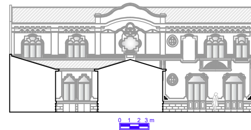
Elevation 03
